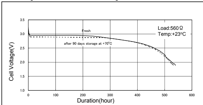
Discharge Characteristics after storage of CR17450E-N
