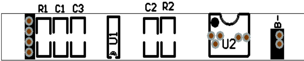
TopLayer (顶层布线图):
