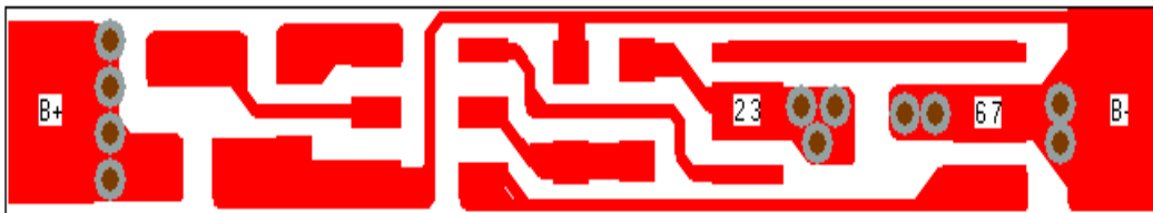
BottomLayer(底层布线图):
